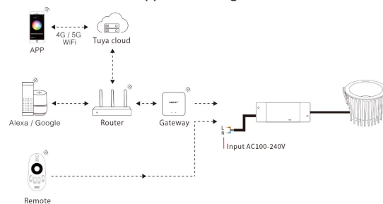
Application Diagram
