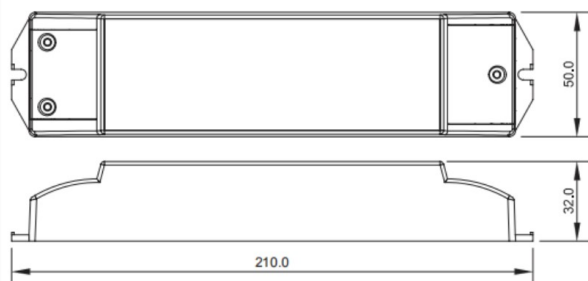
Product Dimension
