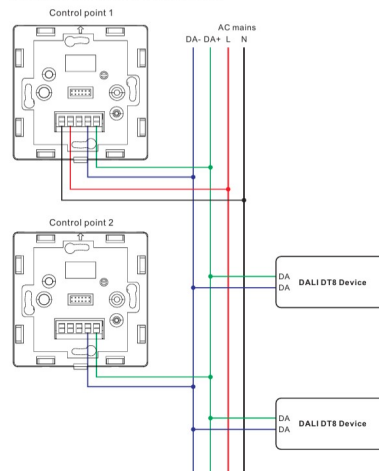
Figure 1: Wiring scheme to control up to 50 DALI ECG via broadcast or control 4 DALI groups.
