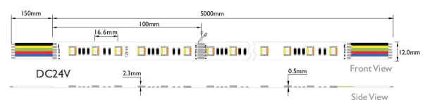
Dimensions(Unit: mm)
