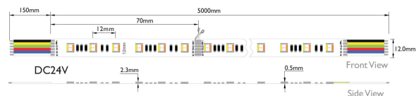
Dimensions(Unit: mm)
