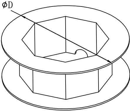
Paper shaft
