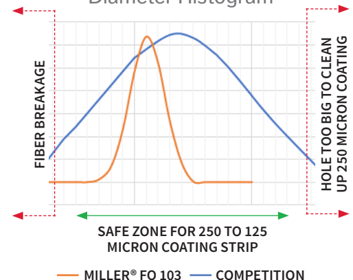
Stripping Hole Nominal Diameter Histogram
