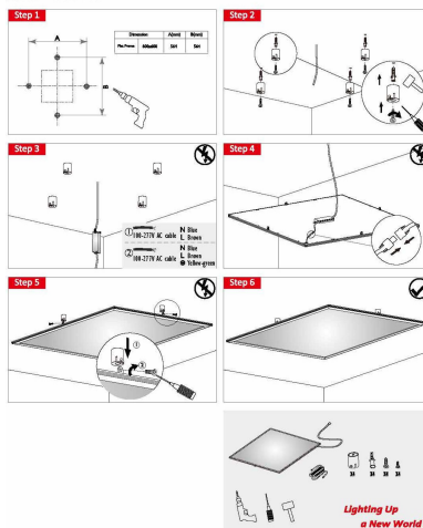
LED Panel Light - Column Surface Mounted
