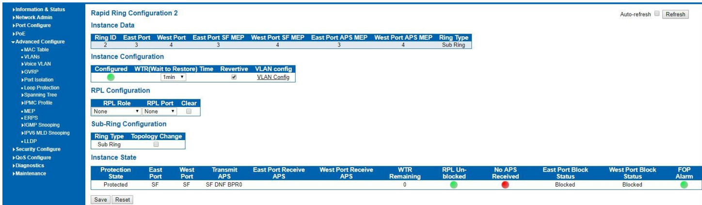
Figure 5-9 EPRS Ring Configuration
