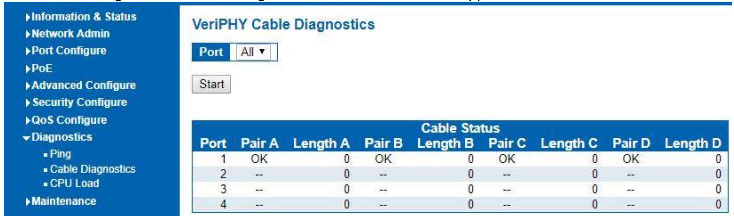
Figure 8-2 Cable Diagnostics Screen
