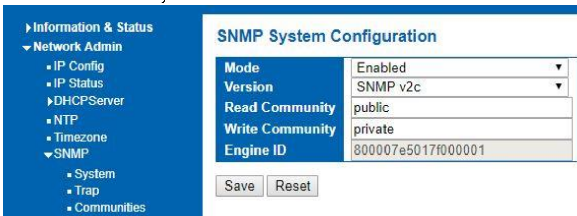
Figure 2-3 SNMP System Setting Screen
