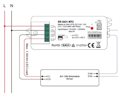
Wiring Diagram
