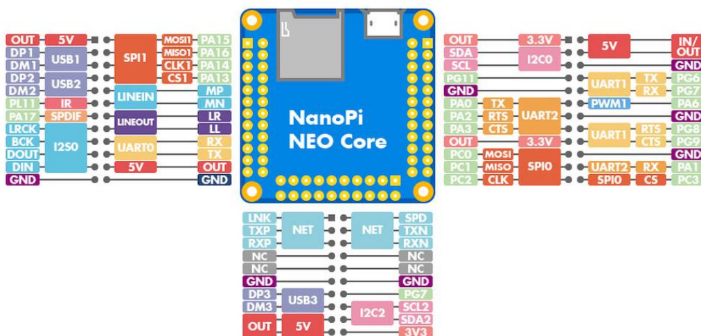
NanoPi NEO Core pinout diagram
