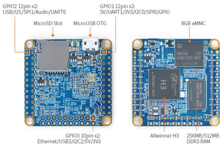
NanoPi NEO Core pinout diagram
