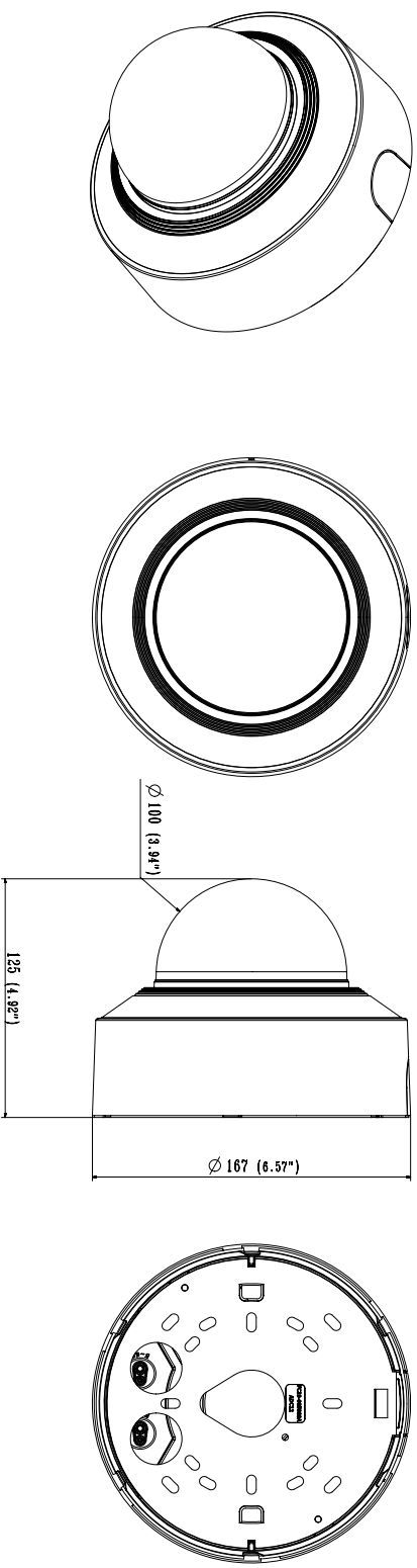
X-PLUS INDOOR VANDAL with SKIN-COVER
